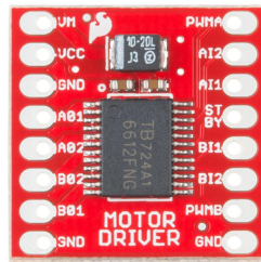
Fig. 16: Driver TB6612FNG Datasheet TB6612FNG
