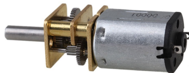
Fig. 14: Motor GA12N20-100 Datasheet GA12N20
